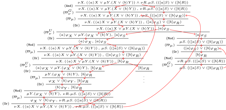
Fig. 2. A tableau for \nu X.(\langle a \rangle X \vee \mu Y.(X \vee \langle b \rangle Y)) \wedge \nu R.\mu S.(\langle a \rangle S \vee \langle b \rangle R)
